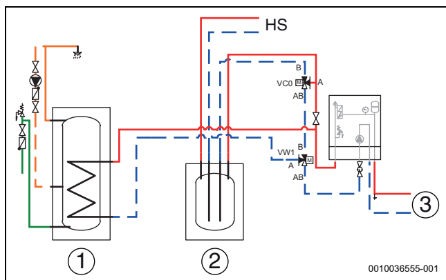
Fig. 30 Akkumulatortank, VC0-bypassventil
